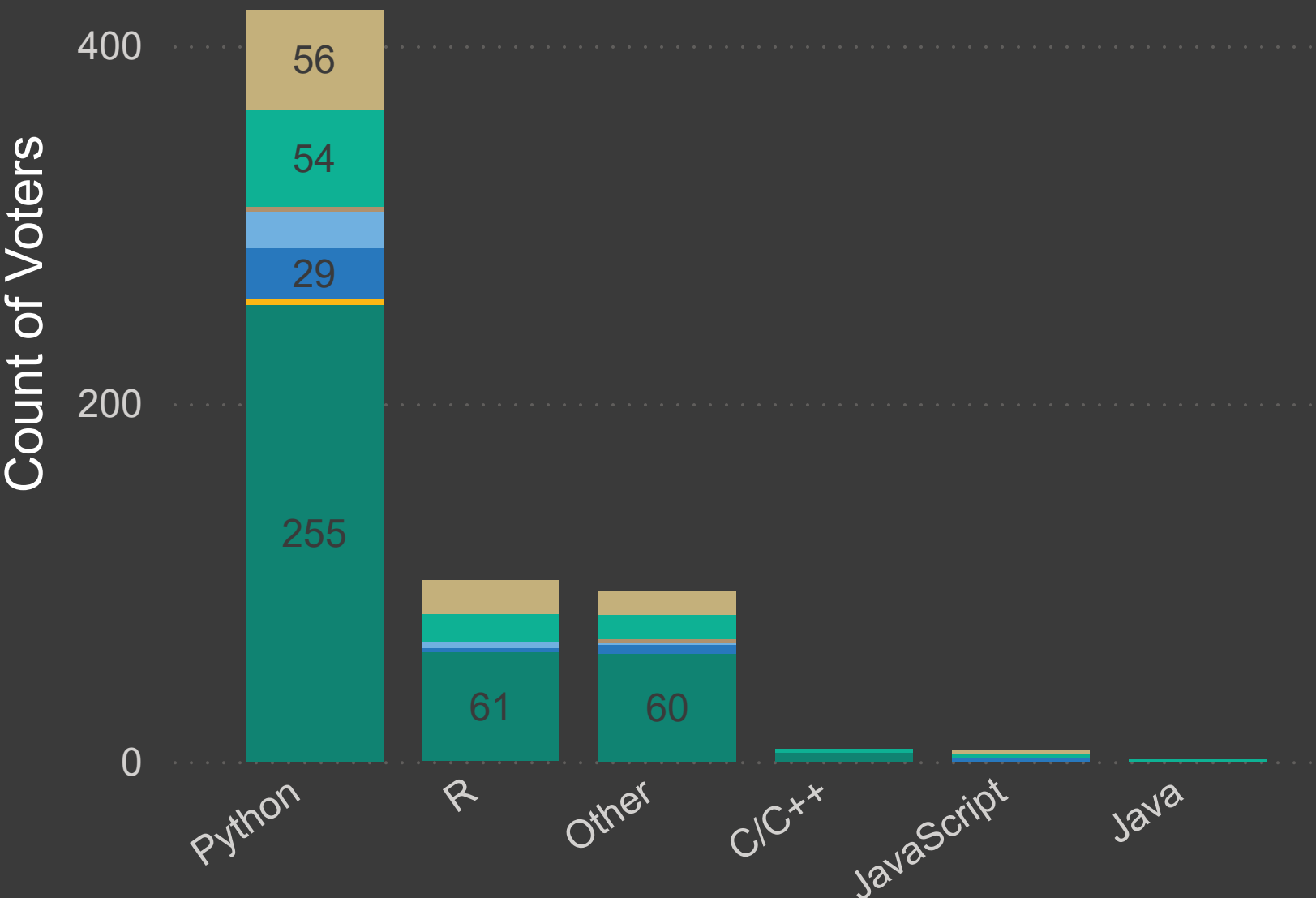
Favorite Programming Language
