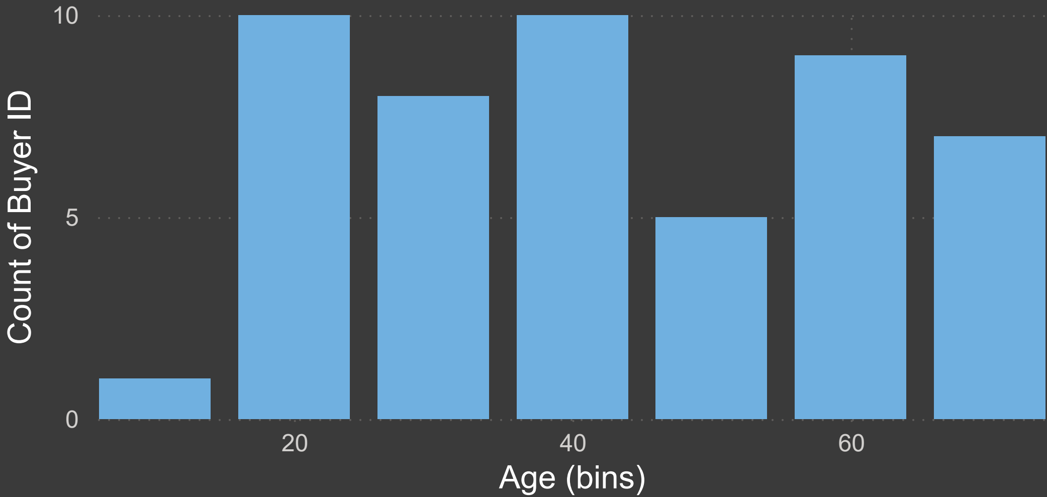
Count of Buyer ID by Age (bins)
