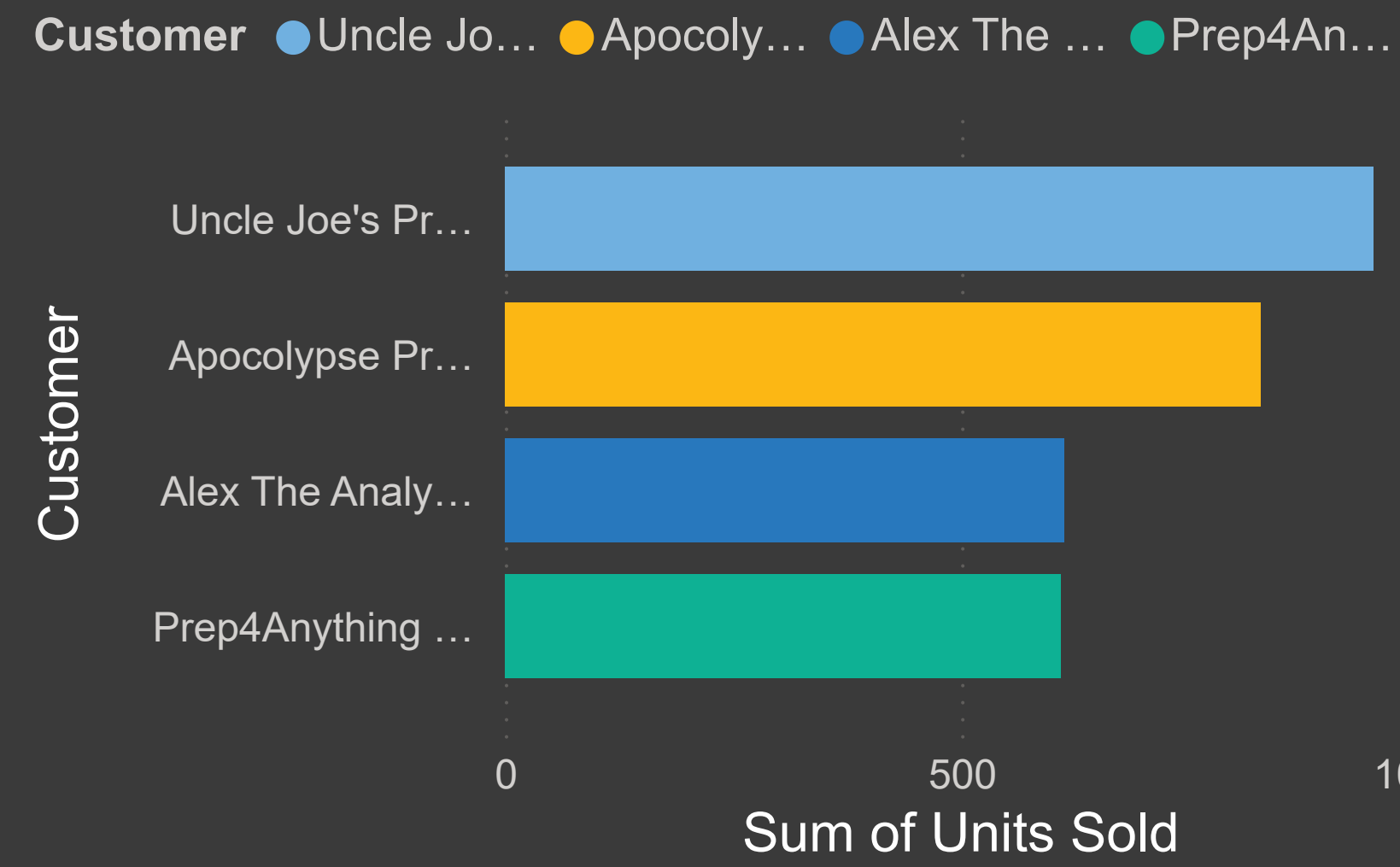
Sum of Units Sold by Customer and Customer
